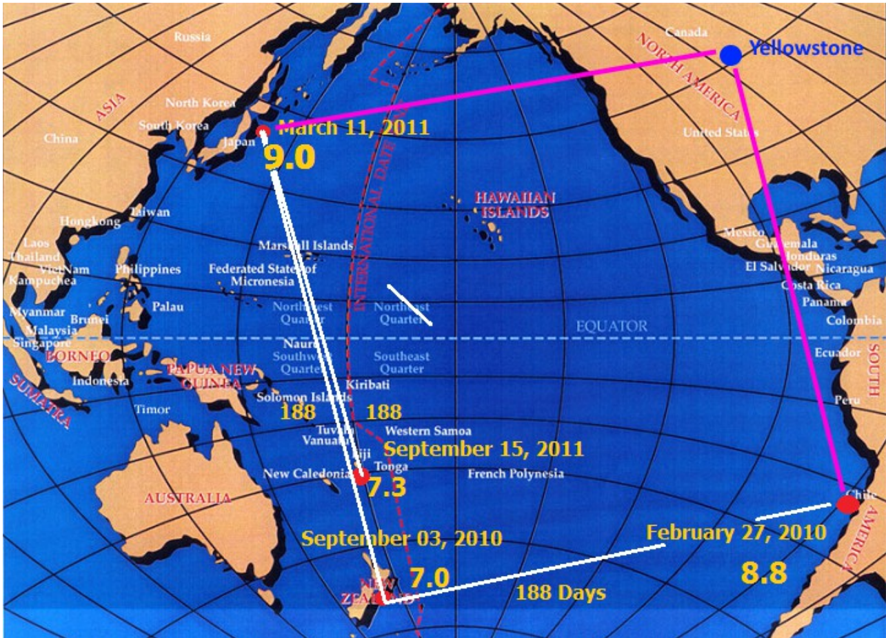
188 days earthquake cycle
