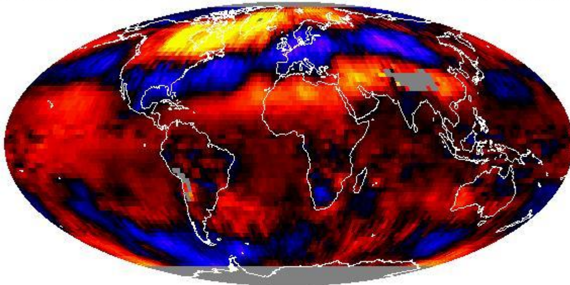
MSU/AMSU Channel TLT Brightness Temperature Anomaly, January, 2010
