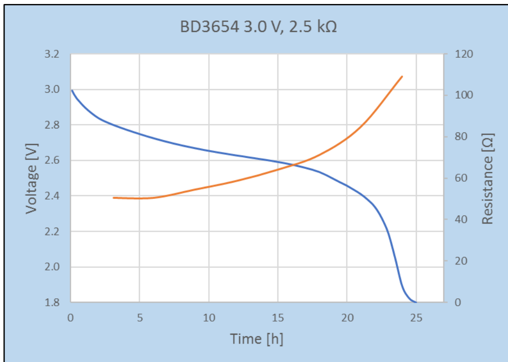
Figure 3. Discharge curve of SoftBattery® BD3654 3.0V with 2.5 k \Omega load at room temperature.
