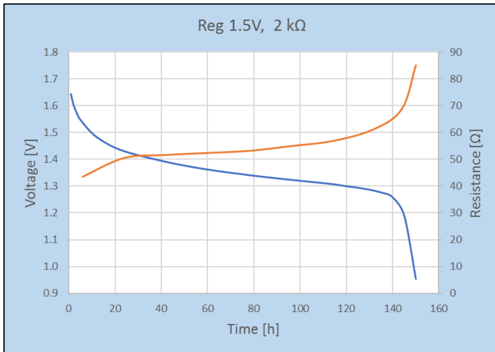
Figure 1. Discharge curve of SoftBattery® Reg 1.5V with 2 kΩ load at room temperature.
