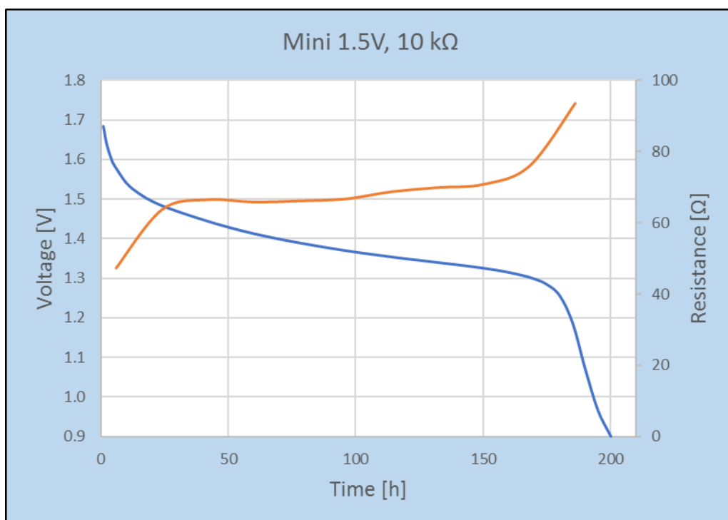
Figure 2. Discharge curve of SoftBattery® Mini 1.5V with 10 kΩ load at room temperature.
