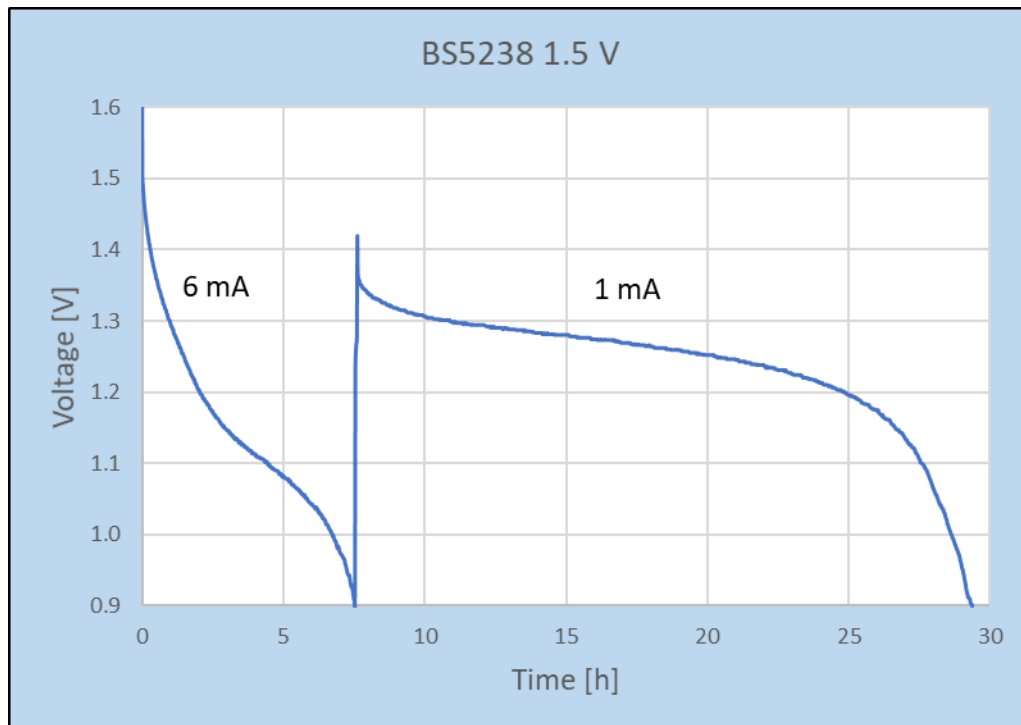
Figure 1. Discharge curve of SoftBattery® BS5238 1.5V with 6 mA load followed by 1 mA load at room temperature.
