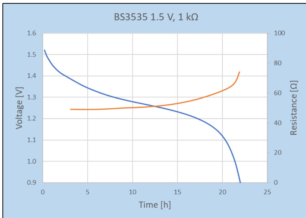
Figure 2. Discharge curve of SoftBattery® BS3535 1.5V with 1 kΩ load at room temperature.
