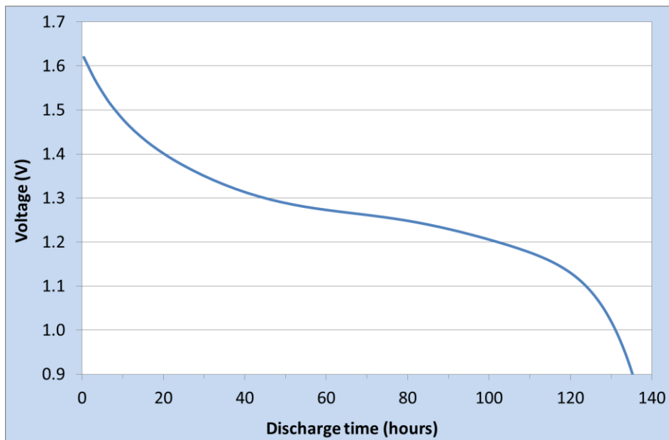
Figure 2. Discharge curves of SoftBattery® Mini 1.5V with 10 kΩ load at room temperature.
