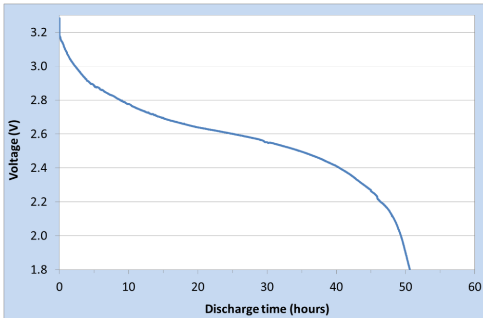
Figure 3. Discharge curves of SoftBattery® Reg 3.0V with 10 k \Omega load at room temperature.
