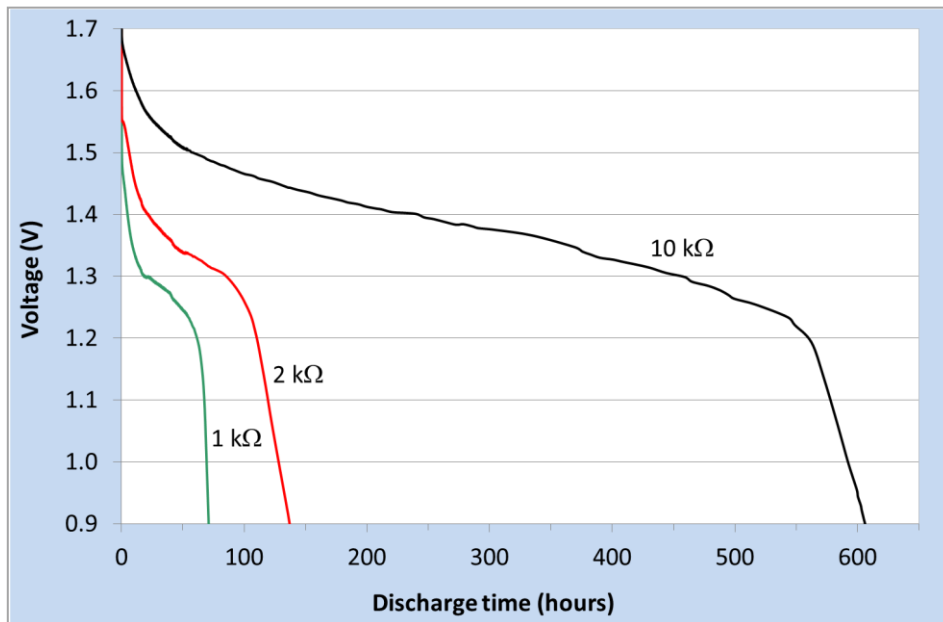
Figure 1. Discharge curves of SoftBattery® Reg 1.5V with various loads at room temperature.
