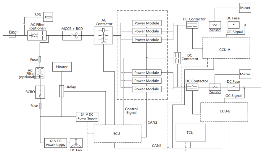
Figure 3-3 Working Principle View
