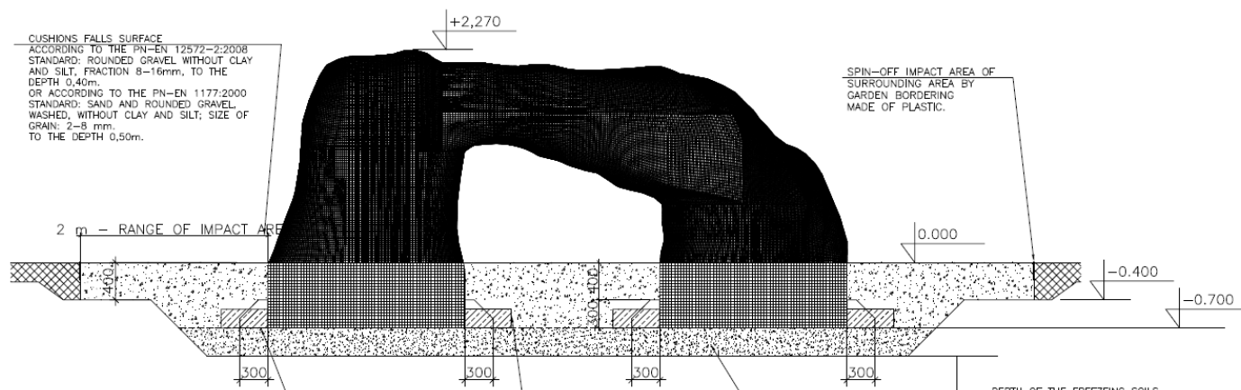
VERTICAL SECTION, FUNDATION OF THE CRAG MDD-006
