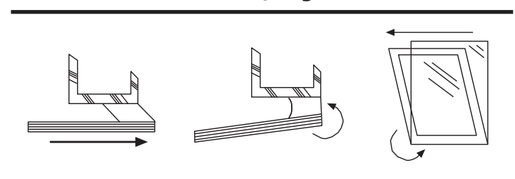
Figure 2: Movement from thermal expansion and contraction and/or glass rotation.
