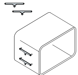
P 783 panel retainer for cases, 1 pair
