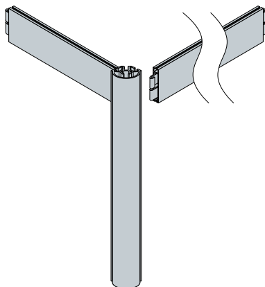
corner solution, version 2 S 1200 extrusion with 90° beam connection, beam extrusion Z 4400
