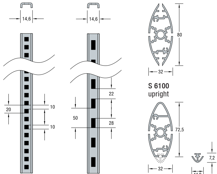
S 6200 slotted insert rail
