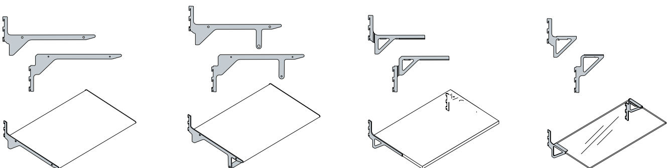
P 700 shelf bracket for postformed shelves, 1 pair
