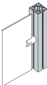
M 1456 panel retainer, panel thickness 4 to 8 mm
